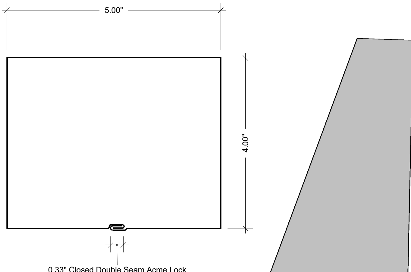
0.33" Closed Double Seam Acme Lock
