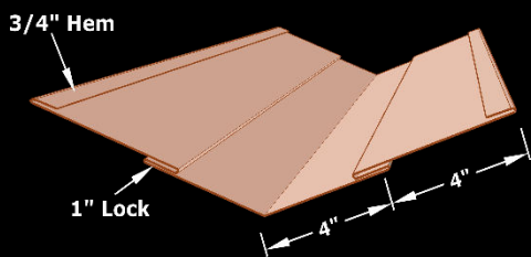
"V" Valley with Panel Lock for Standing Seam
