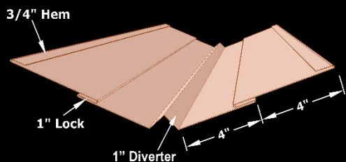
"W" Valley with Panel Lock for Standing Seam
