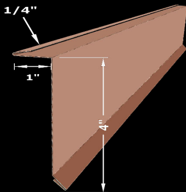
Counter Flashing
