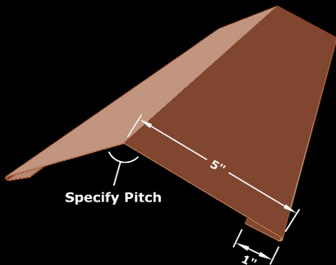
Hip & Ridge Cap
