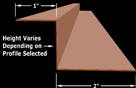
"Z" Flashing
